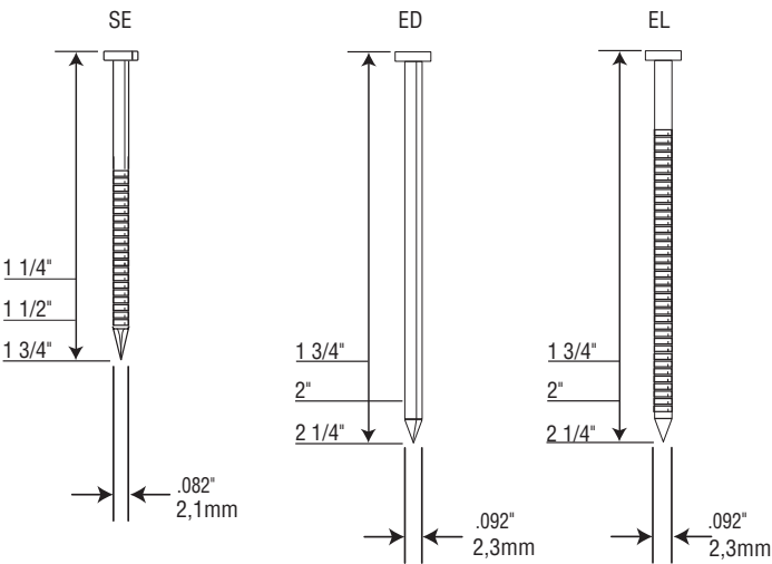
15 Degree Wire Welded or Plastic Carrier Coil
